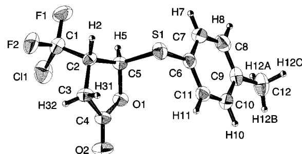
Figure 1. ORTEP view of (2 R ,3 S )- 7c showing the atomic labeling scheme
